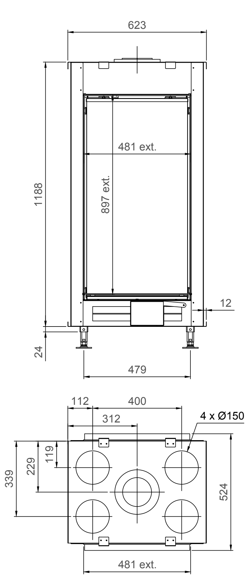
LUNA Diamond 550DV GAS
